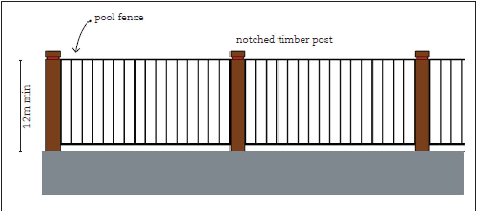
Figure 14 - Fencing Detail 4 - Green Infrastructure Zone
